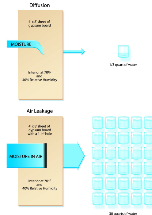
Figure 1: Moisture Transport via Diffusion vs. Air Leakage
